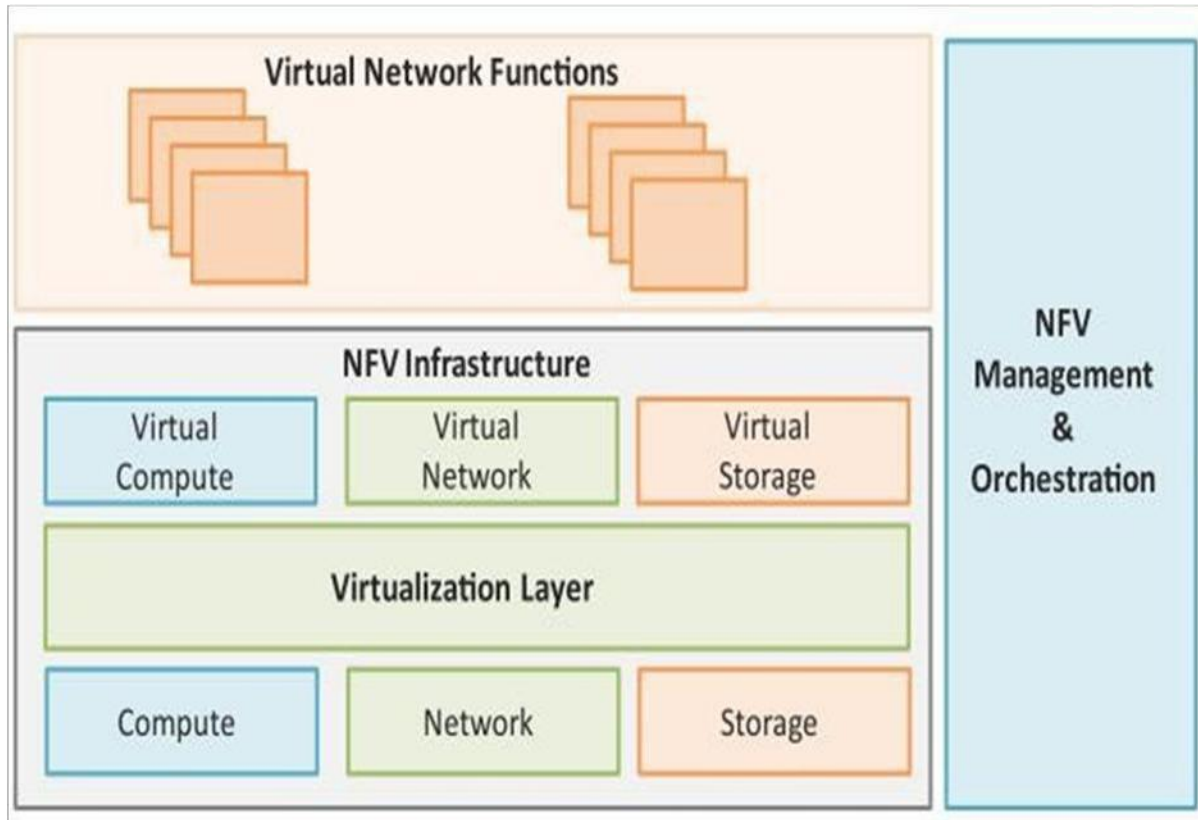
NFV Architecture
