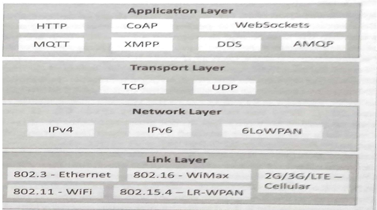
Fig 1.4 IOT Protocols
