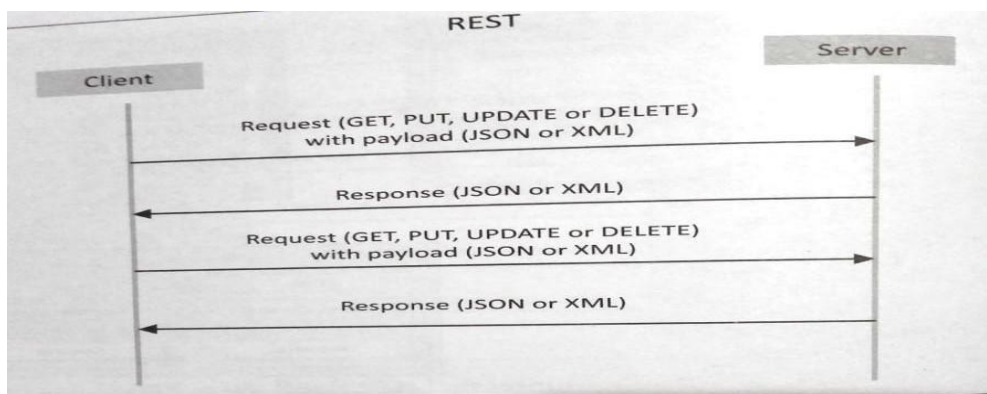
Fig 1.4 Request-Response model
